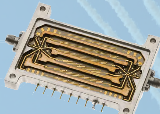
6 CHANNEL FILTER BANK
