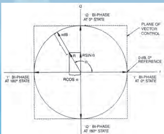
VECTOR MODULATOR
