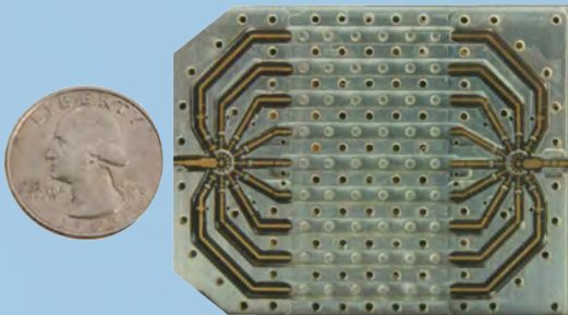
9 CHANNEL FILTER BANK
