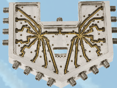
SP16T SWITCH
